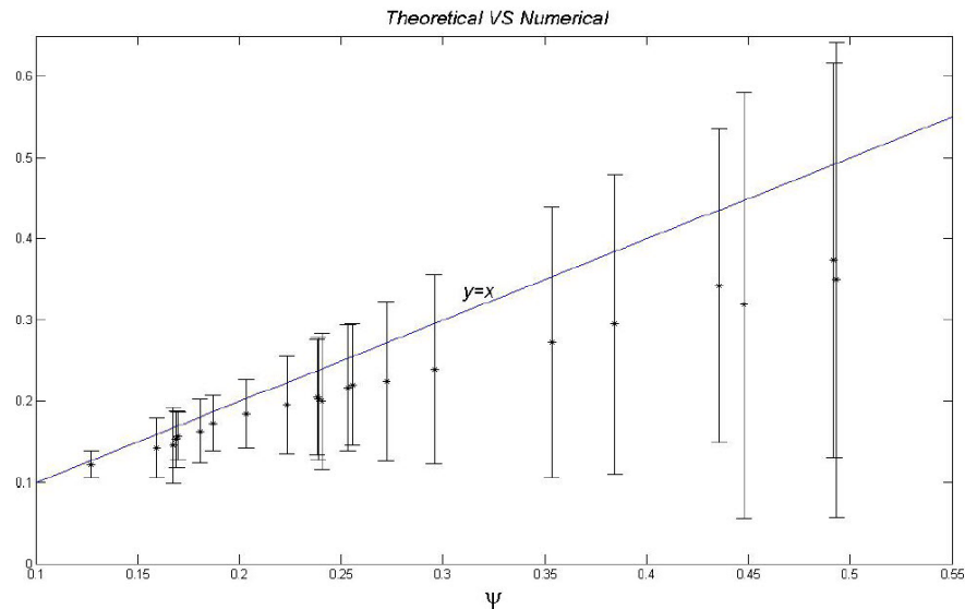
Figure 1 Plot of theoretical value of storage computed from (16) versus value of storage computed numerically.
